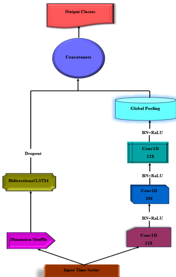
Fig. 2. BiLSTM-FCN Model
