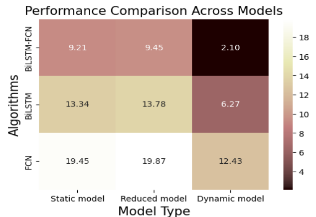
Fig. 6. Performance Comparison
