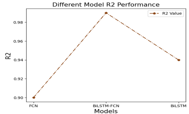
Fig. 3. Performance of R^2
