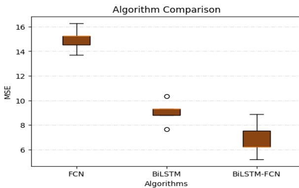
Fig. 5. Comparison of the MSE
