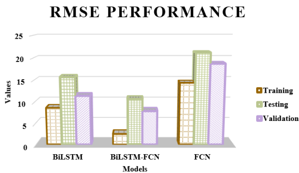
Fig. 7. RMSE Performance
