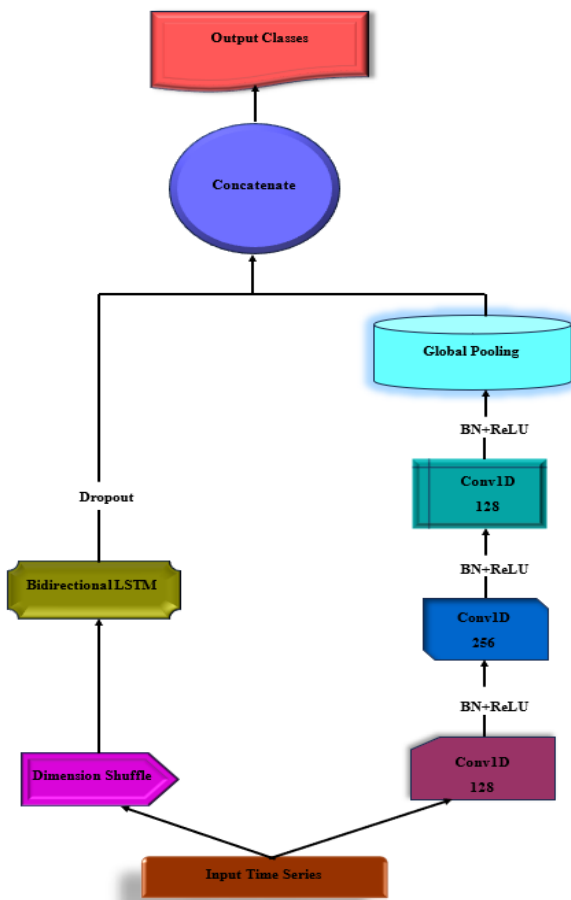
Fig. 2. BiLSTM-FCN Model
