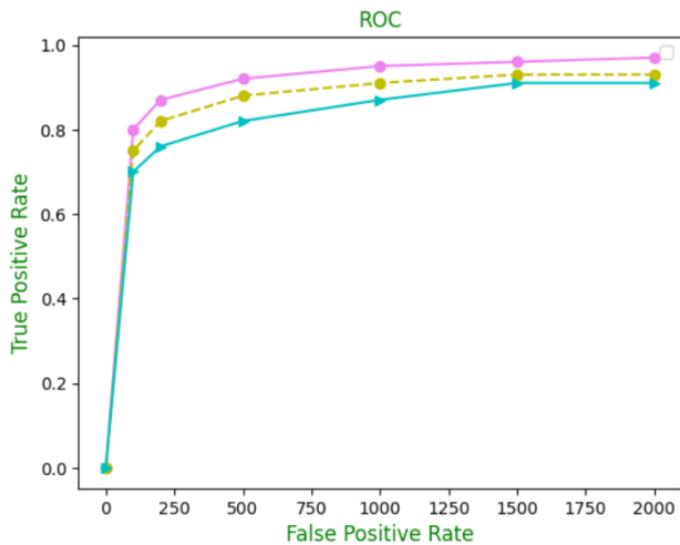
Fig. 2. ROC Curves
