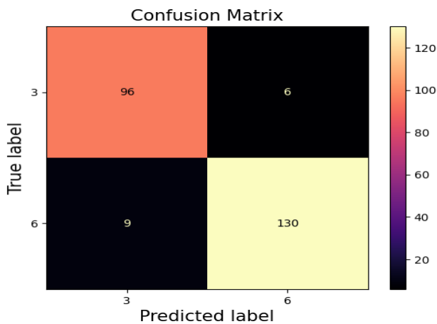
Fig. 3. Confusion Matrix
